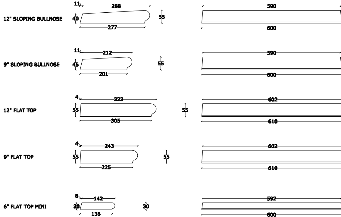
SECTION
